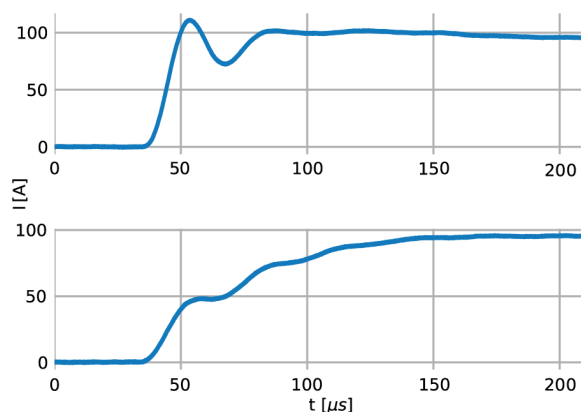
Figure 2: Parameterization example of a 36 kW, 1000 V, 108 A device: Set-value step current 0...97 A@333VDC in <50 \mu s with overshoot (top), in <200 \mu s w/o overshoot (bottom). This dynamic behavior is characteristic for all G5 devices.
