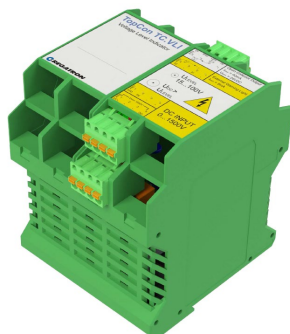
Figure 8: The VLI unit is positioned next to the DC connection point. The unit provides both an LED on the module and an interface for the external LED, which is placed on the front of the system.
