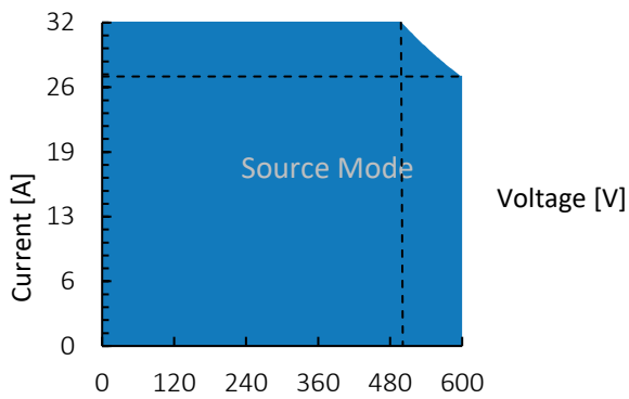
Figure 1: TC.P.16.600.400.S, voltage / current operating area.
