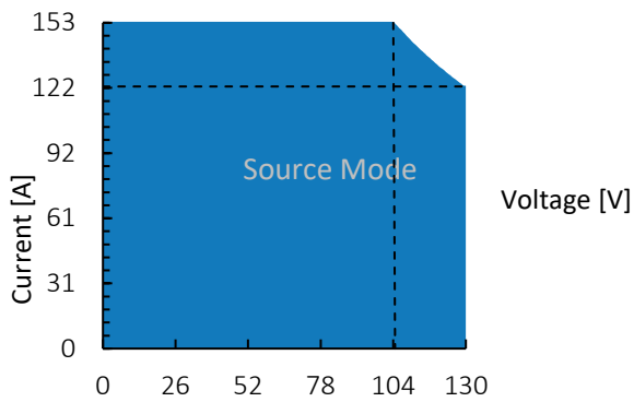
Figure 1: TC.P.16.130.400.S, voltage / current operating area.
