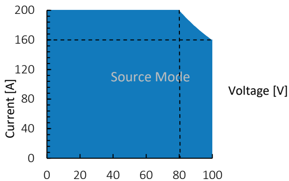
Figure 1: TC.P.16.100.400.S, voltage / current operating area.
