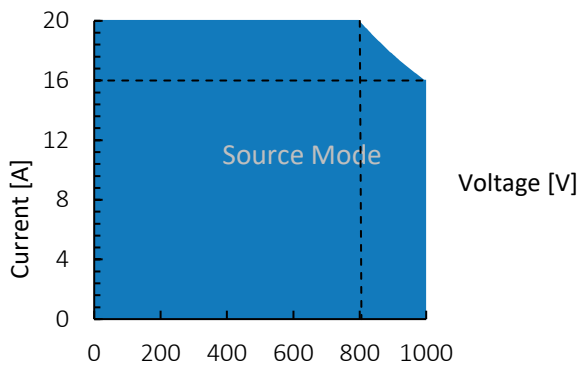
Figure 1: TC.P.16.1000.400.S, voltage / current operating area.
