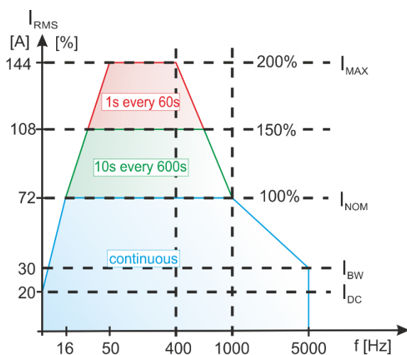
Figure 3: Overloadability versus frequency
