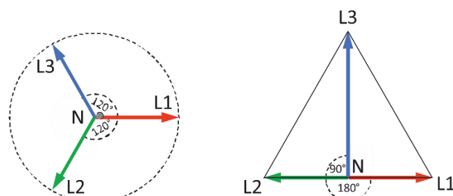
Figure 6: 3L + N
