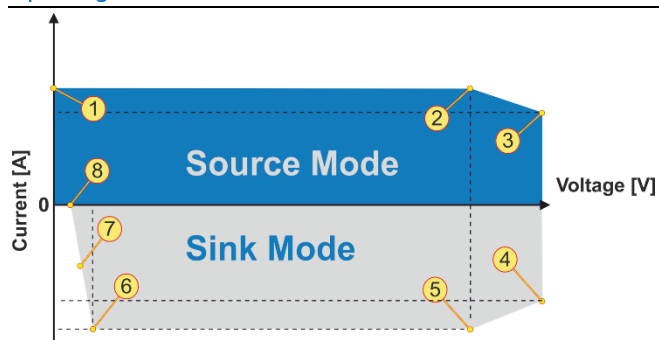
Figure 1: TC.GSS. 32. 65.4WR.S, voltage/current operating area
