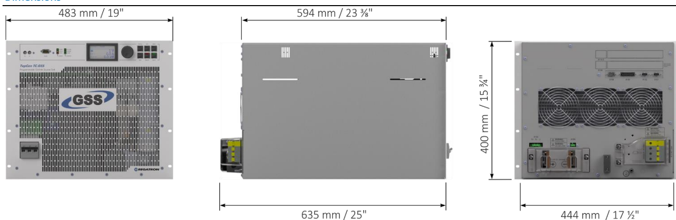
Figure 2: Front, right hand side and rear view. 19-inch module with 9 units in height.
