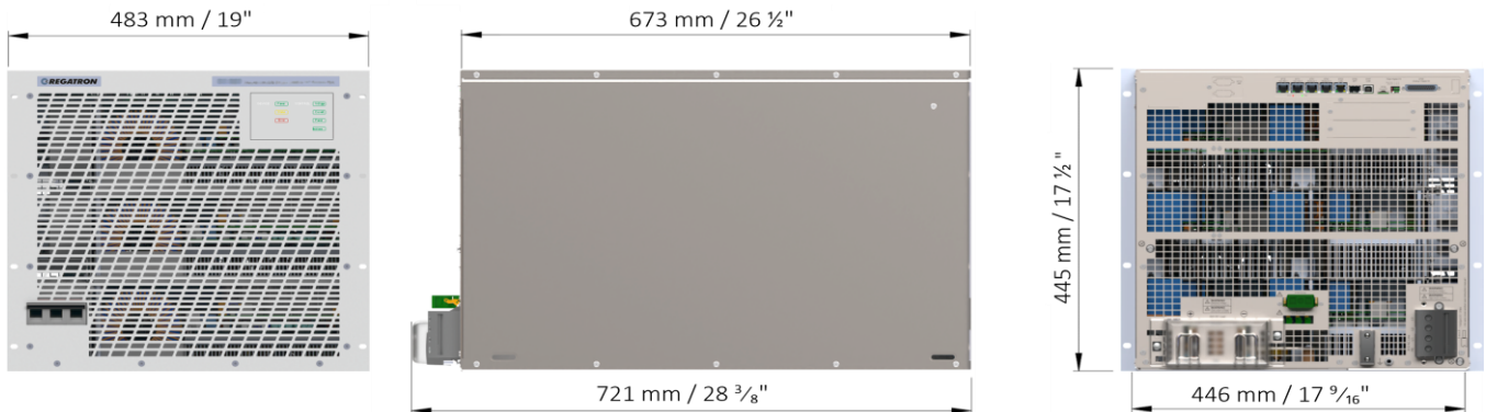
Figure 3: Front, right hand side and rear view. 19-inch module with 10 units in height.
