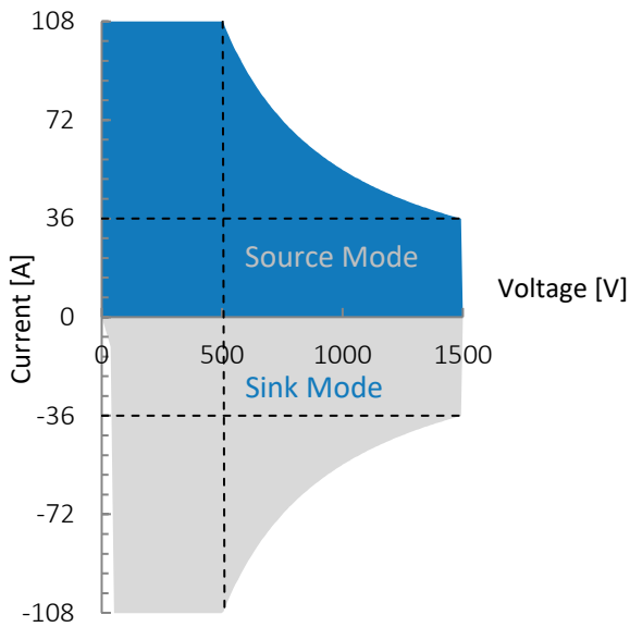
Figure 1: G5.IND.54.1500.108, voltage/current operating area.
