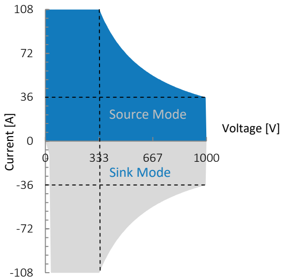
Figure 1: G5.IND.36.1000.108, voltage/current operating area.
