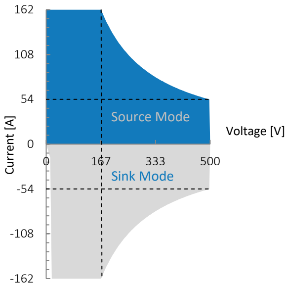
Figure 1: G5.IND.27.500.162, voltage/current operating area.
