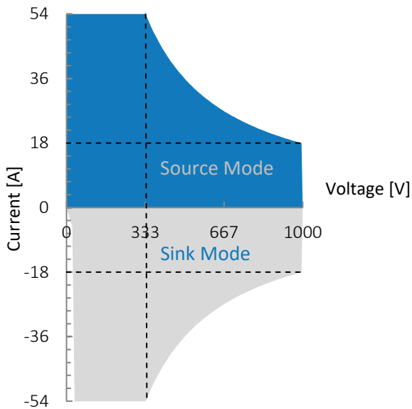
Figure 1: G5.IND.18.1000.54, voltage/current operating area.
