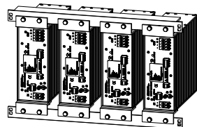
Figure 2. 19"-rack mounting
