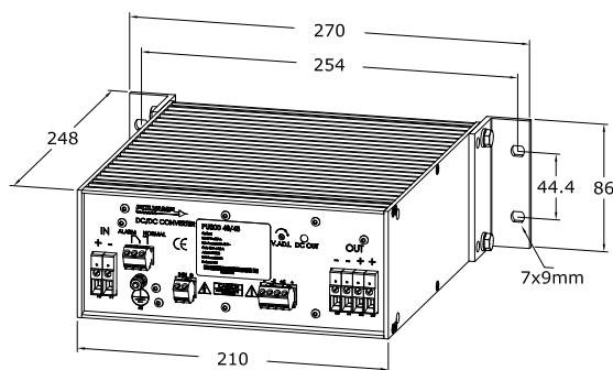
Figure 1. Dimensions
