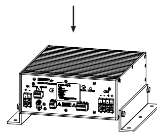
Figure 3. Wall and chassis mounting
