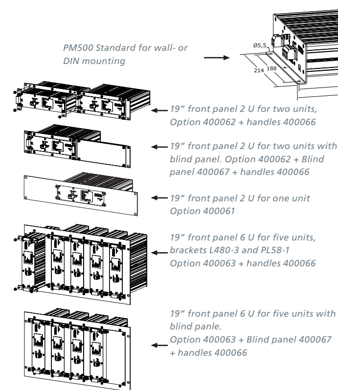
Figure 2. 19"-rack mounting PM500 R
