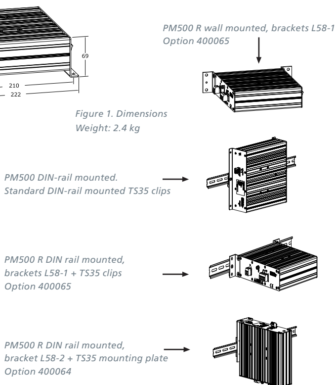
Figure 4. Wall, chassis & DIN mounting
