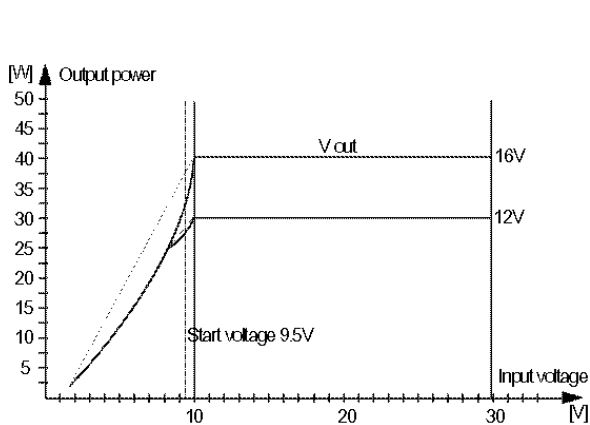
Figure 5. Output power PM50A15-15
