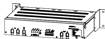
Figure 3. Wall mounting
