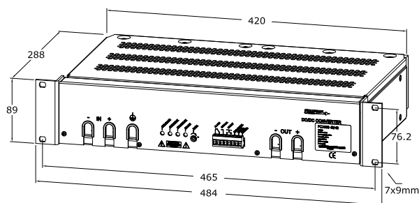
Figure 1. Dimensions
