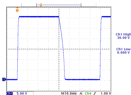
SM66-AR-110 with Power Sink Option fast discharge of output capacitors by Power Sink circuit
