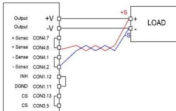
Configuration Remote Sense Mode
