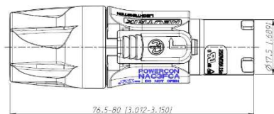
Neutrik NAC3FXXA-W-S
