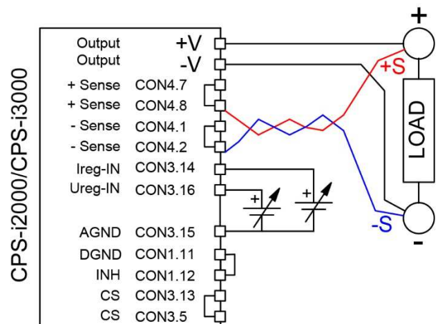
Remote Sense Configuration
