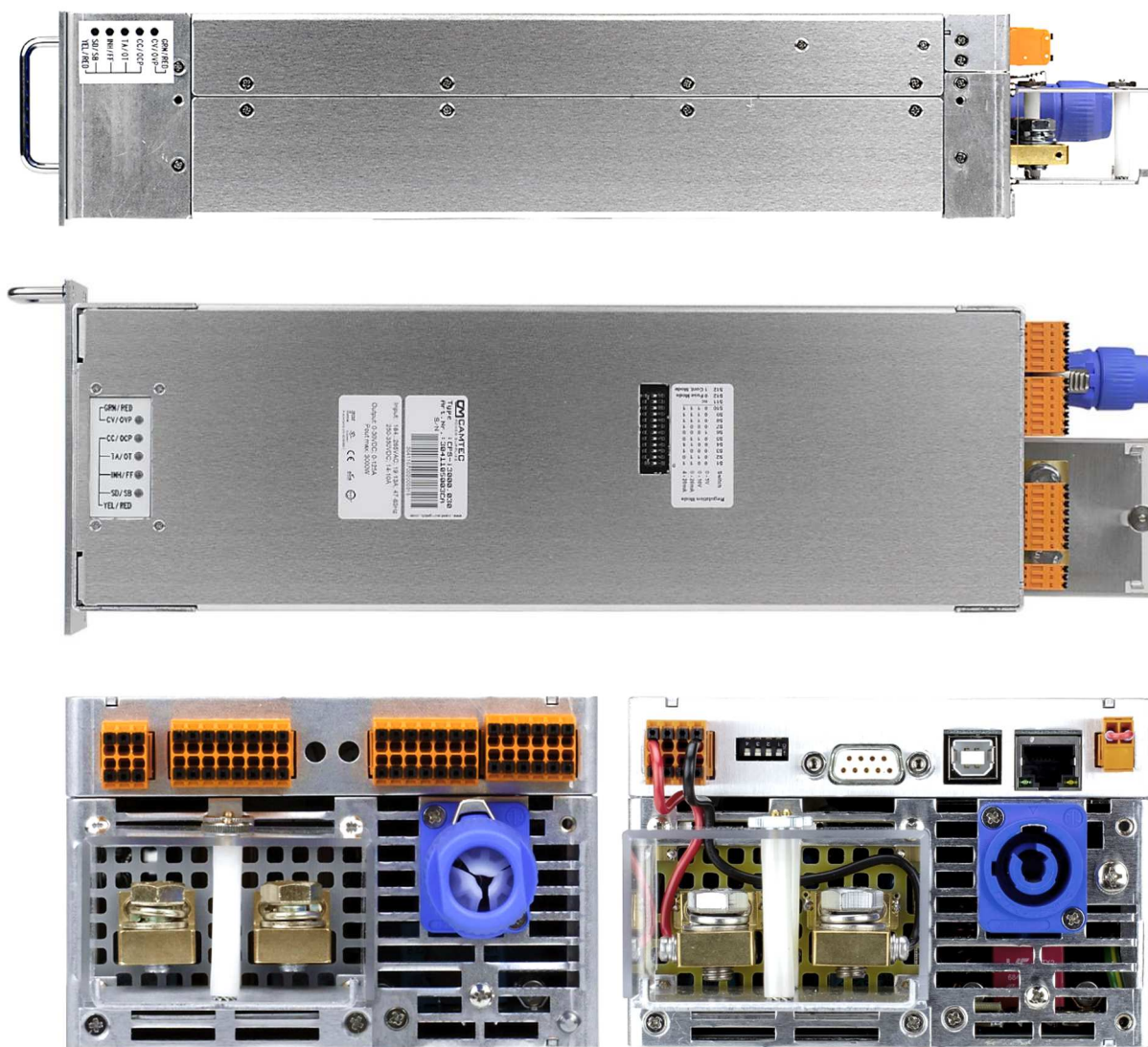
ANALOGUE INTERFACE
