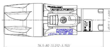
Neutrik NAC3FXXA-W-S
