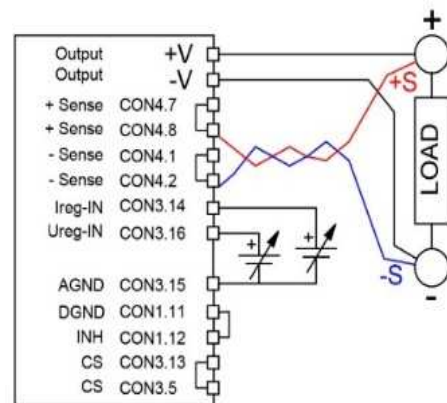
Remote Sense Configuration
