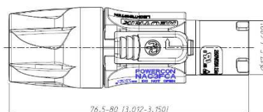
Neutrik NAC3FCA
