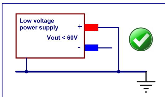
Fig 2: Plus DC power terminal connected to Protective Earth.
