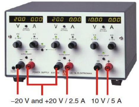
fig. 3 - 2 Dual Voltage Tracking Mode
