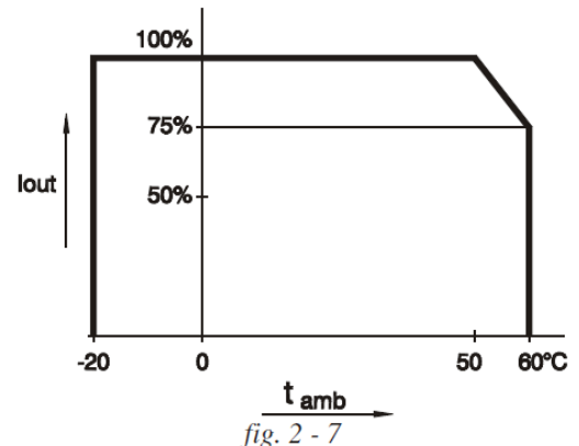
fig. 2 - 7 Operating temperature ranges
