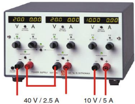
fig. 3 - 3 Series Tracking Mode
