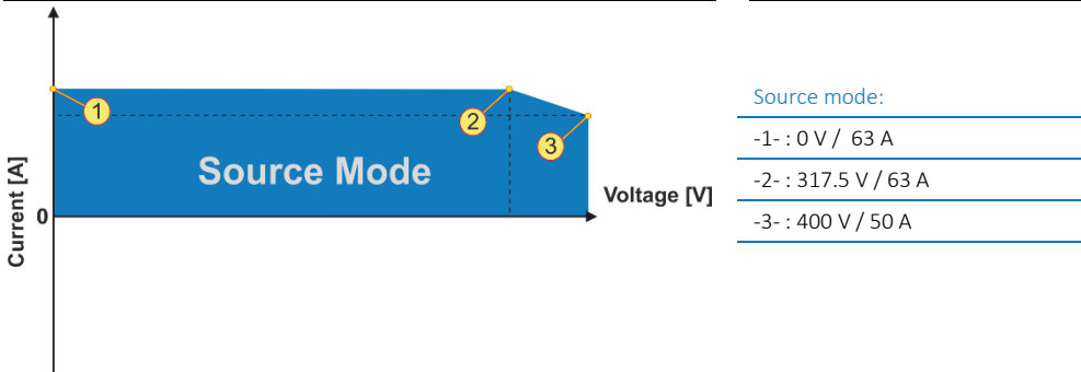
Figure 1: TC.GSX.20.400.4WR.S, voltage/current operating area
