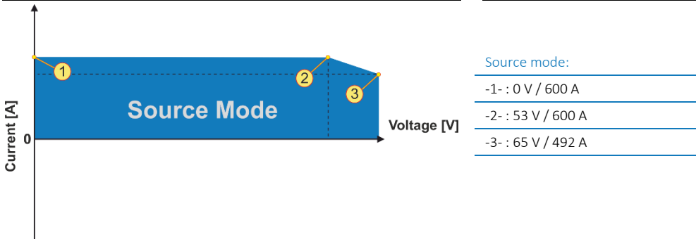
Figure 1: TC.GSX.32.65.4WR.S, voltage/current operating area
