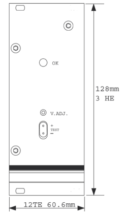
Figure 8. Front panel 3HE option L
