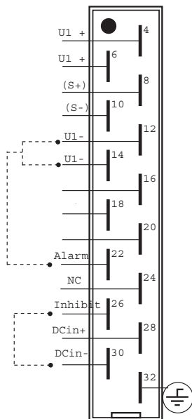
Figure 1. Pin-out single output with connector DIN41612, H15.
