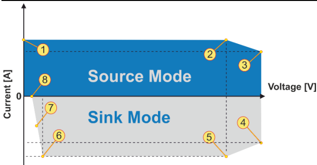
Figure 1: TC.GSS. 32. 500.4WR.S, voltage/current operating area
