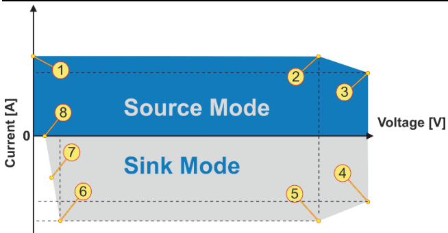
Figure 1: TC.GSS. 20. 65.4WR.S, voltage/current operating area
